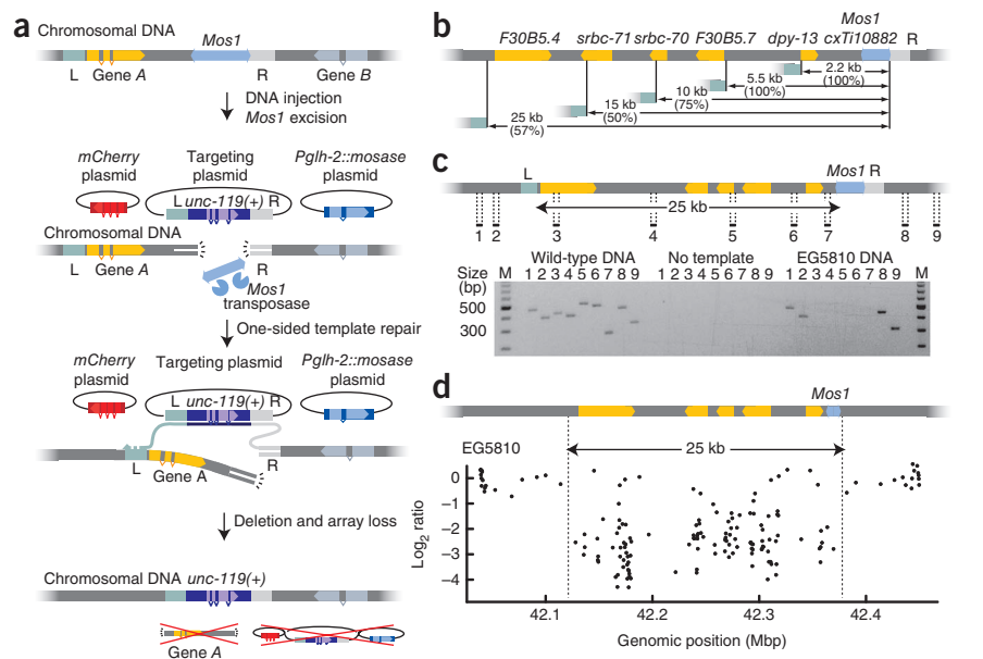
Figure 1 | Using Mos1 transposons to create targeted deletions. (a) Schematic of MosDEL.
